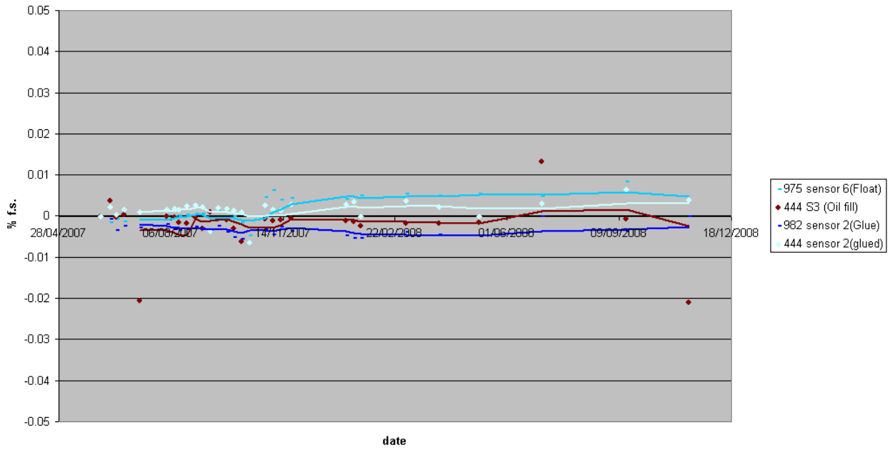
Fig 5 Full scale output stability
