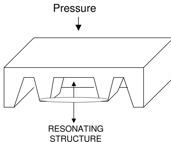
Fig 1 Resonant pressure sensor operation
