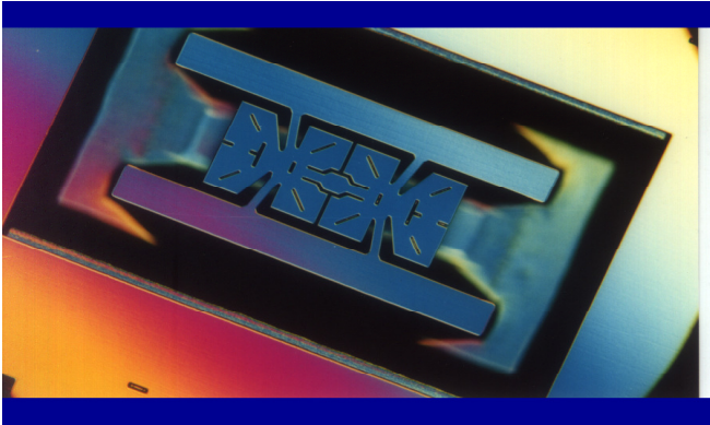
Fig 2 GE Druck RPT single crystal silicon element.
