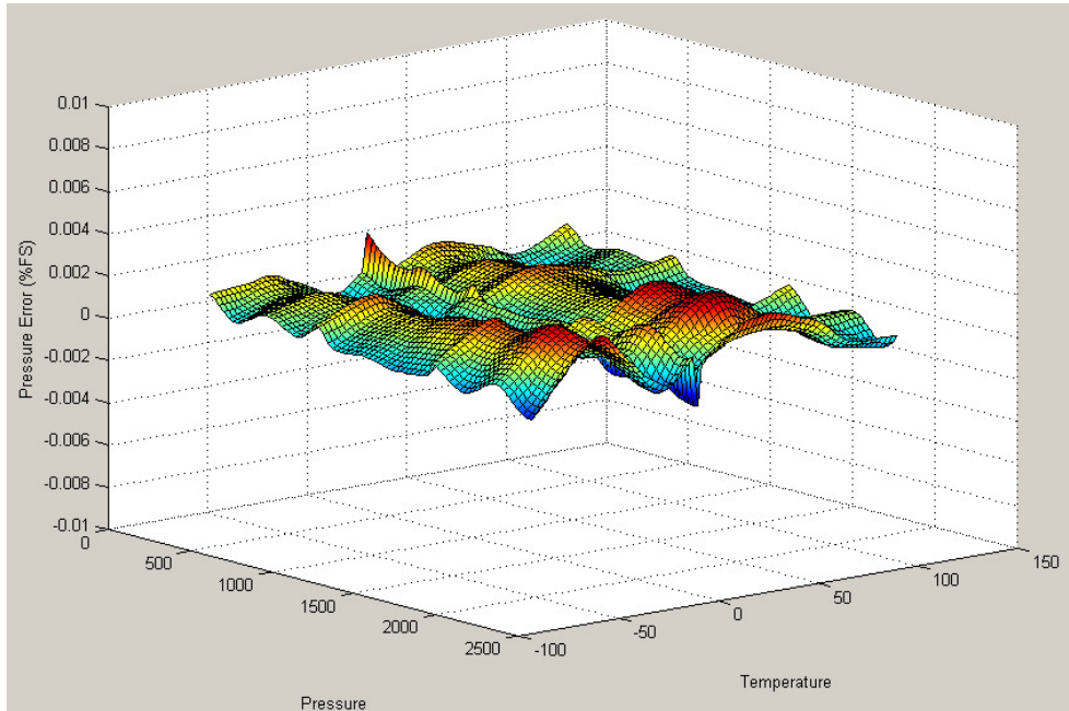
Fig 6 Curve-fit accuracy
