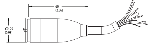
DEPTH CABLE
