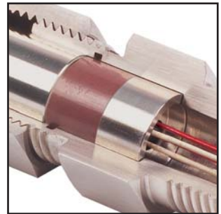
Spectite® sealed feedthroughs have a wide operating temperature range.
